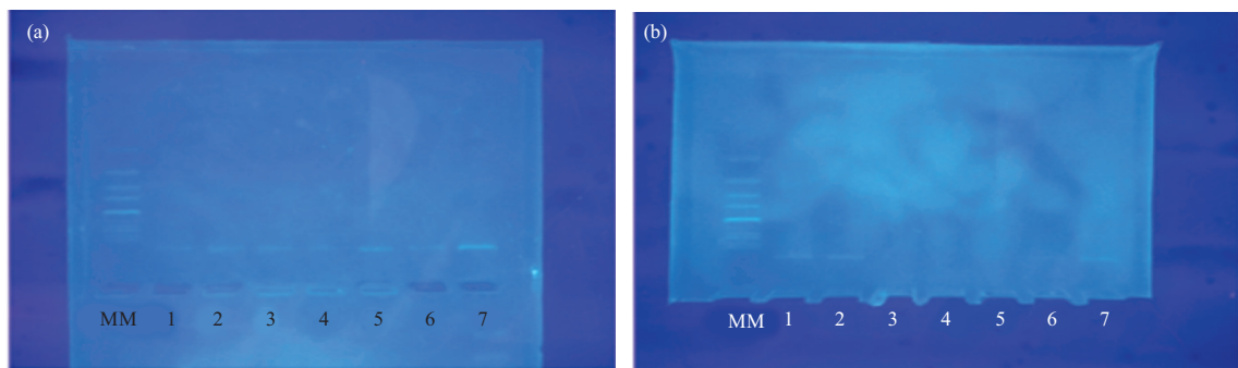
Fig. 1: Gel electrophoretic pattern of DNA from (a) Preserved and (b) Discarded blood sample
